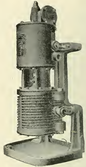
3/4 INCH PUMP MOUNTED ON SPECIAL STAND WITH DRIP PAN.
